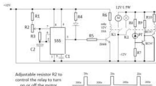
Figure 7. Schematic diagram to control operation of trap
