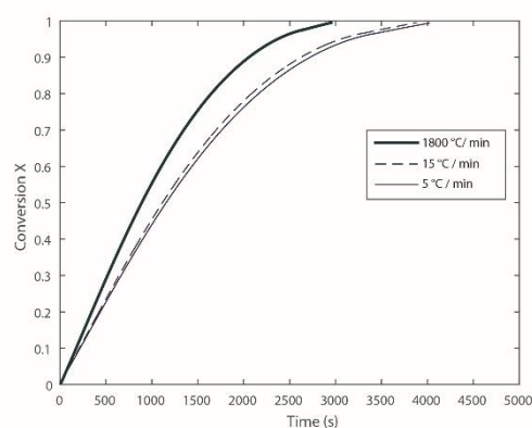
Figure 3. Influence of heating rate on gasification kinetics
