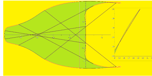
Figure 1. The absolute stability region of the AB4-BDF4
