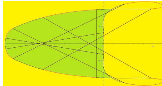
Figure 2. The absolute stability region of the AB4-BDF3
