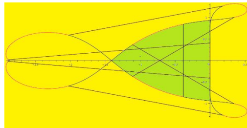
Figure 4. The absolute stability region of the AB4-AM4
