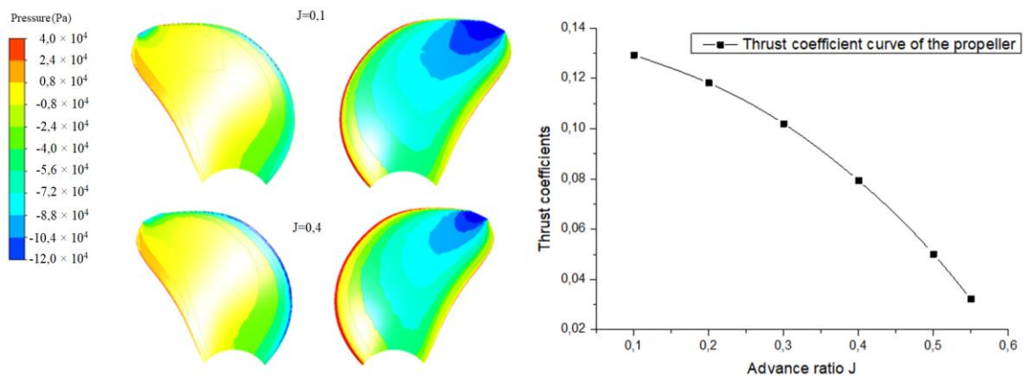
Figure 3. Pressure distribution faces of propeller at J of 0,1; 0,4 and changing law of propeller's thrust coefficient
