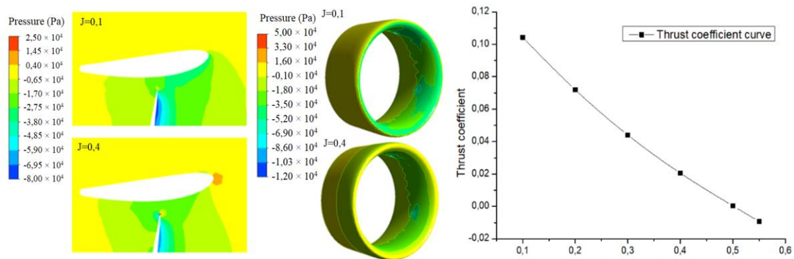
Figure 2. Pressure distribution on the duct at J = 0,1; 0,4 and changing law of thrust coefficients
