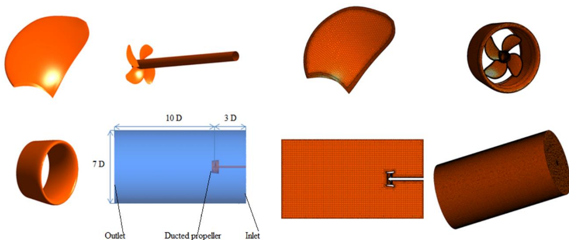
Figure 1. Duct, propeller, investigated domain and mesh
