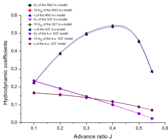
Figure 7. Hydrodynamic performance of the ducted propeller with different turbulent models
