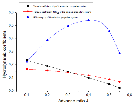
Figure 5. Thrust, torque, efficiency coefficient of the ducted propeller
