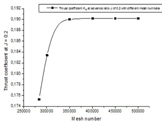
Figure 1. Results of mesh independence and detail parameters of mesh
