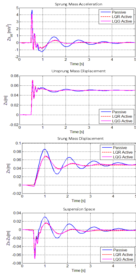
Figure 6. Time response of \ddot{Z}_s, Z_s, Z_u, Z_s - Z_u with the step road profile
