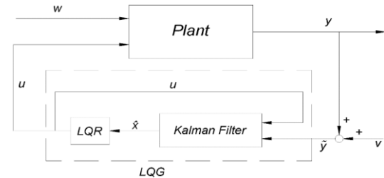
Figure 5. LQG controller diagram
