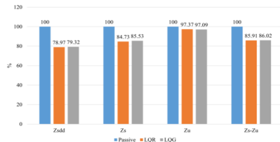
Figure 7. RMS of \ddot{Z}_s, Z_s, Z_u, Z_s - Z_u with the step road profile
