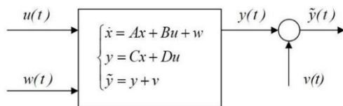
Figure 2. Linear system changes continuously over time with noise and measurement noise
