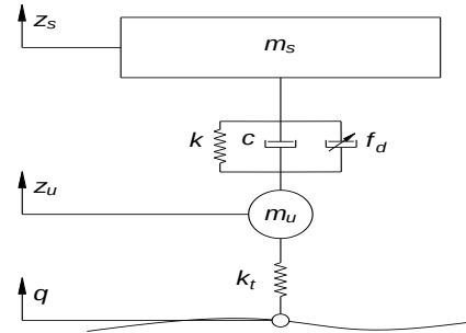
Figure 1. Quarter vehicle model
