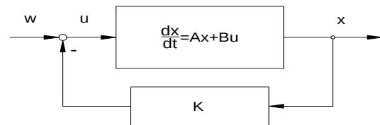
Figure 4. Feedback controller design diagram
