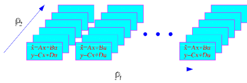
Figure 4. LPV models defined on a rectangular grid
