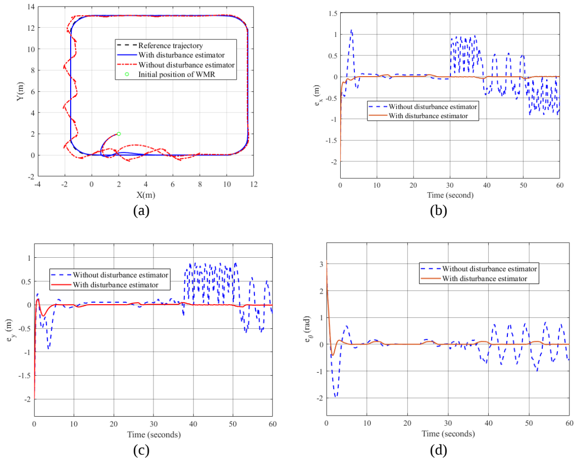
Figure 3. Comparison of the proposed method to the case without disturbance estimator. (a) WMR's trajectories, (b) control errors for x , (c) control errors for y , (d) control errors for orientation angle \theta .
