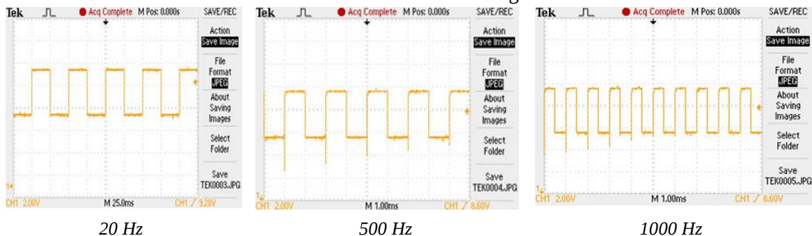
Figure 5. Pulse patterns at different frequencies when the laser module operating in the pulse modes
