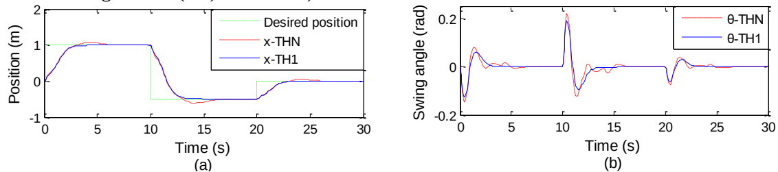
Figure 10. The characteristic curve (a): of the response to the position of the forklift, (b): and the angle of the load in the presence of noise
