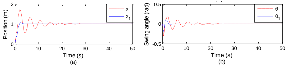
Figure 4. The characteristic curve (a): for the position of the forklift, (b): the swing angle of the load
