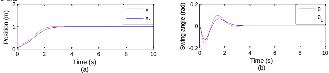
Figure 8. The characteristic curve (a): for the position of the forklift, (b): the swing angle of the load
