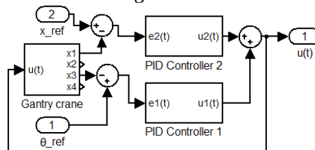
Figure 7. Structure diagram of matlab using dual PID controllers to control crane gantry for CE
