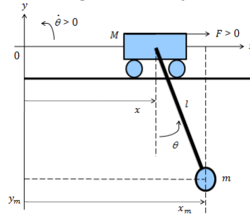
Figure 2. Diagram of the gantry crane system for the CE
