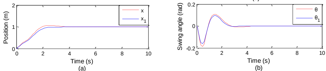
Figure 5. The characteristic curve (a): for the position of the forklift, (b): the swing angle of the load
