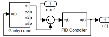
Figure 3. Structure diagram of matlab using a PID controller to control a gantry crane for CE
