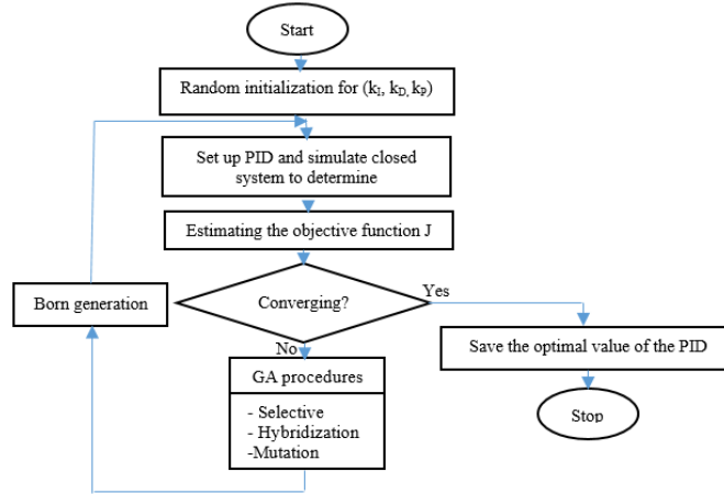
Figure 6. Flowchart of the GA process algorithm to determine the parameters of the PID controller
