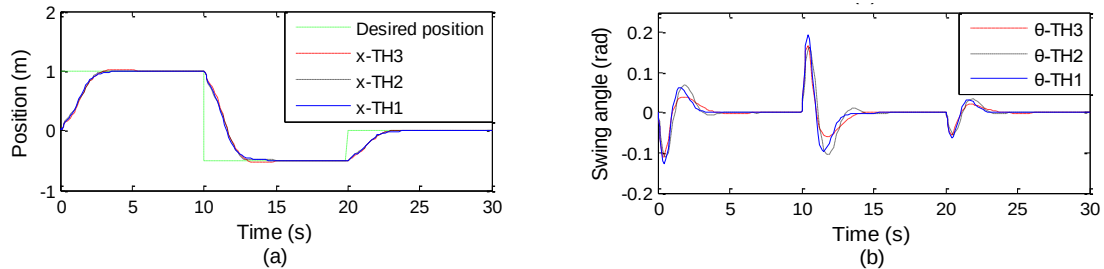
Figure 9. The characteristic curve (a): of the response of the forklift's position, (b): the swing angle of the load when changing system parameters
