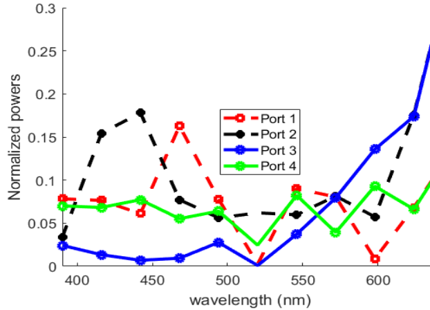
Figure 8. Normalized power at ports 1-4 over the wavelength RGB
