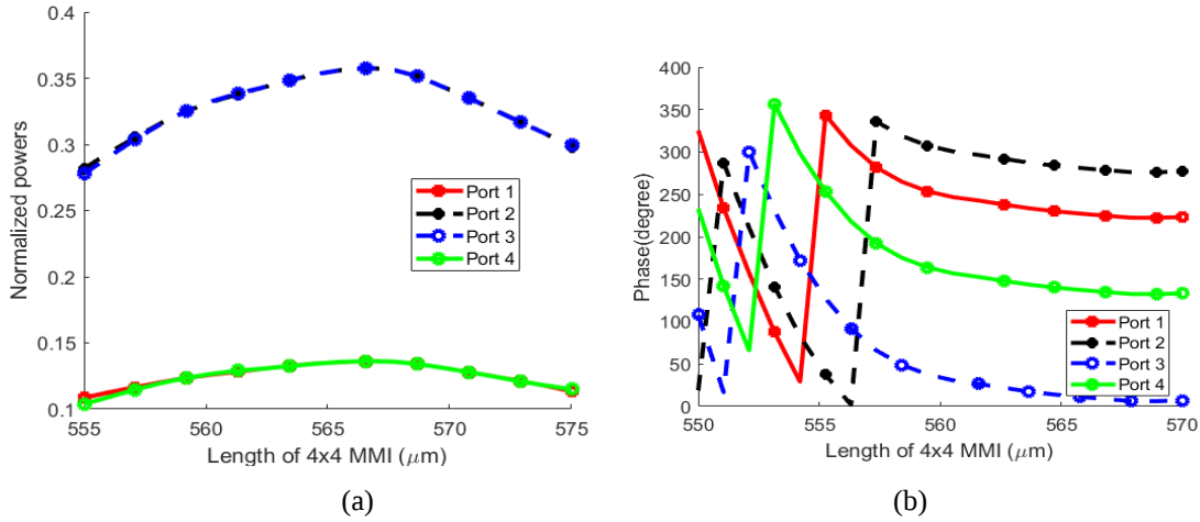
Figure 7. (a) Normalized power and (b) Phase at output ports of the KLT transform
