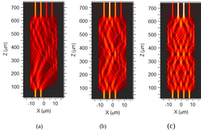
Figure 5. Simulation result of the KLT for different image data with 2, 3 and 4 inputs
