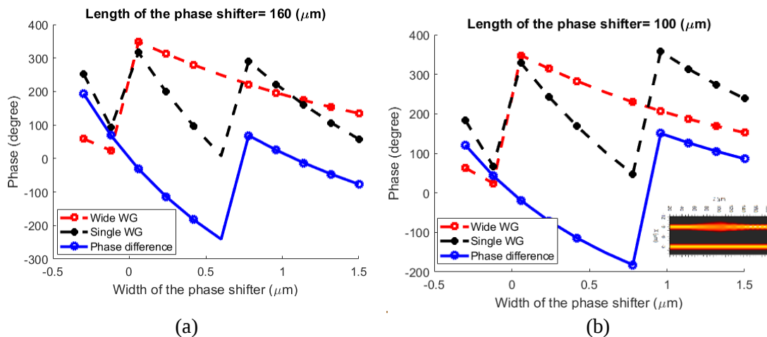
Figure 6. Phase shifts achieved from the wide waveguide (a) with a length of 160\mu\text{m} and (b) length of 100\mu\text{m}
