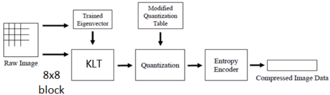
Figure 3. Principle of the image compression using the KLT transform
