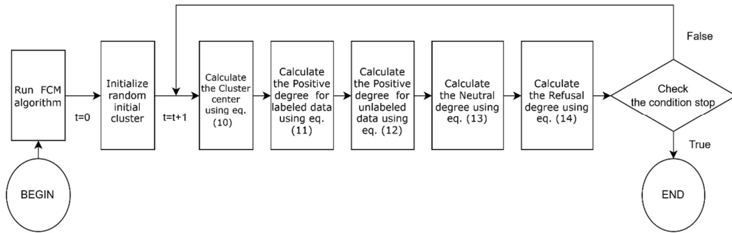
Figure 1. The algorithm diagram of NPFS3FCM
