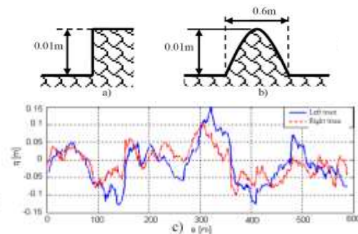
Figure 8. Road profiles: a) Step profile, b) Sine wave profile, c) Random profile
