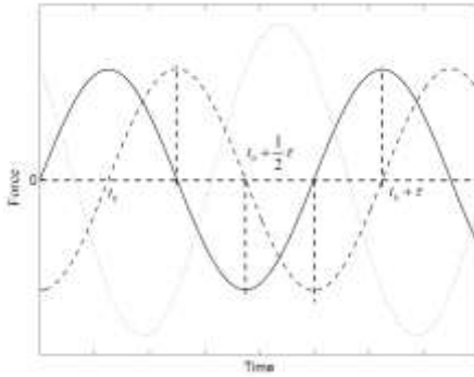
Figure 4. Relation between the forces acting on the sprung mass “m” in case of an harmonized excitation: _____ : Damping force ( F_d ); - - - - - : Spring force ( F_k ) and ..... : Inertial force ( m\ddot{x} )
