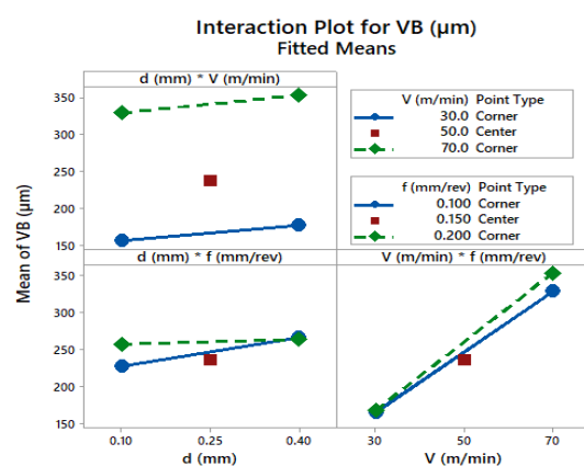
Figure 8. The interaction effects of the cutting parameters to the flank wear
