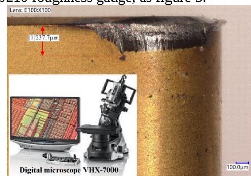
Figure 4. Flank wear measured by digital microscope VHX7000
