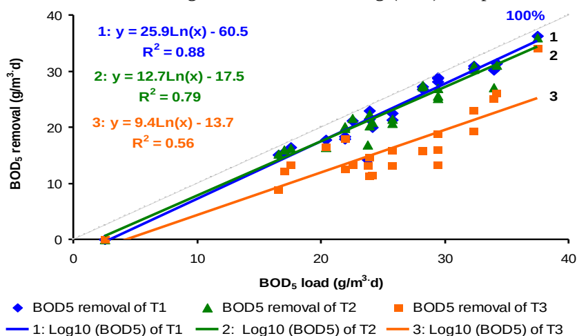
Figure 8. Comparison of \text{BOD}_5 removal with \text{BOD}_5 load into the reactors
