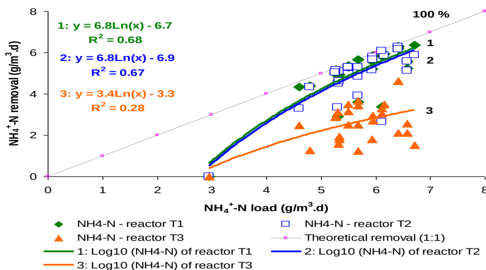
Figure 3. The evaluation of \text{NH}_4^+\text{-N} load and \text{NH}_4^+\text{-N} removal rate of the reactors
