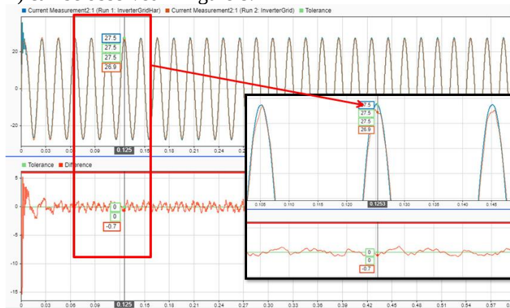
Figure 7. Differential output current value before and after filter improvement
