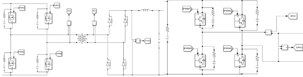
Figure 2. Modeling of DC/DC PSFB combined Full-Bridge inverter unit in Simulink
