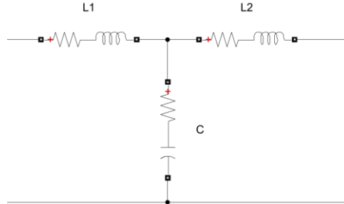
Figure 3. LCL filter in Simulink
