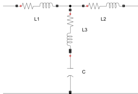
Figure 4. LLCL filter in Simulink
