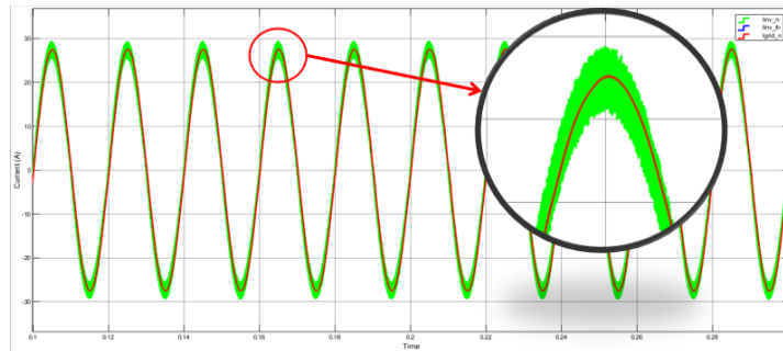
Figure 6. Output current waveform of inverter with LLCL filter
