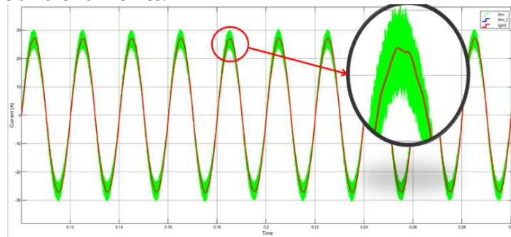
Figure 5. Output current waveform of inverter with LCL filter
