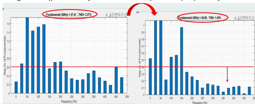
Figure 8. THD comparison between LCL and LLCL filters
