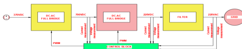
Figure 1. Block diagram of grid-connected inverter [5], [6]
